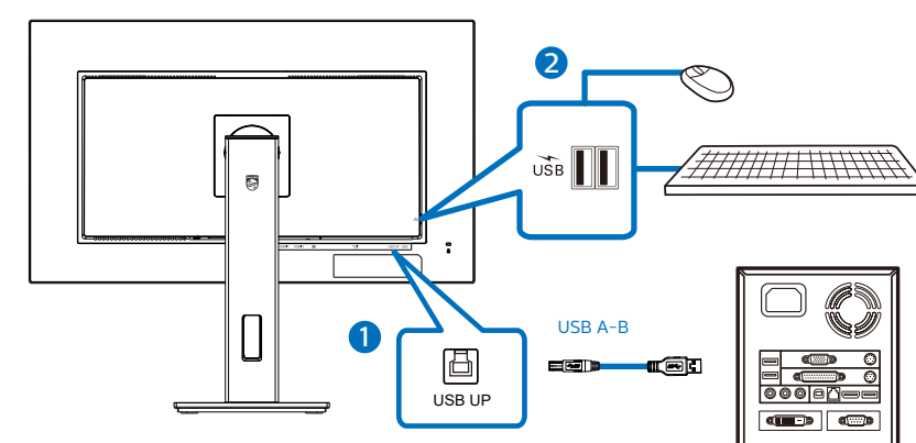
USB hub
