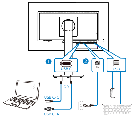
USB docking
