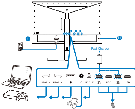
USB Hub
