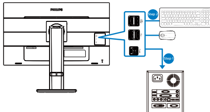
USB hub
