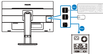
USB hub
