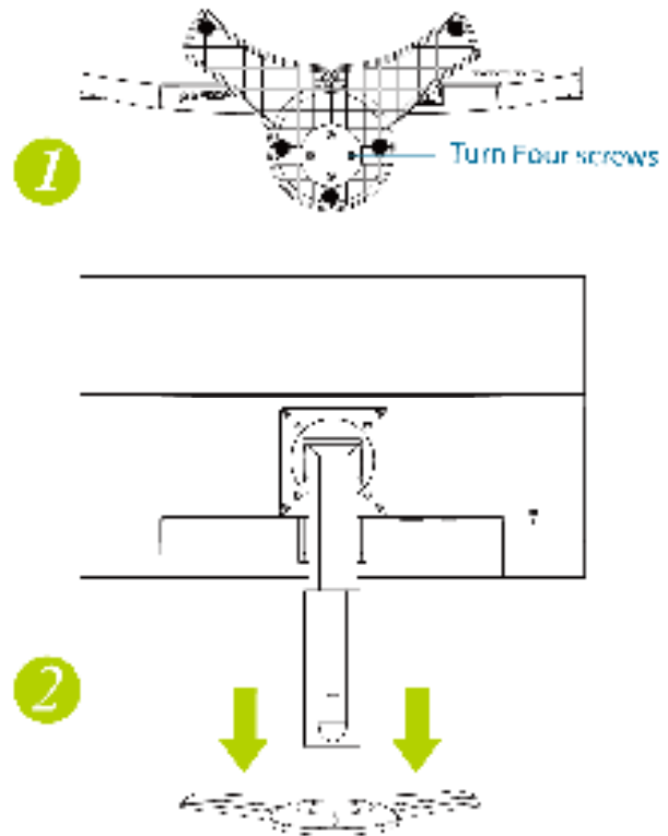
Figure.1. Installing and Removing the Base
