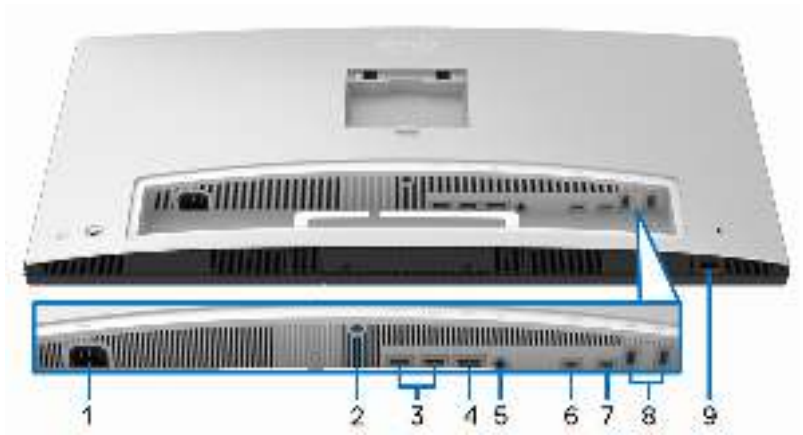
Bottom view without monitor stand
