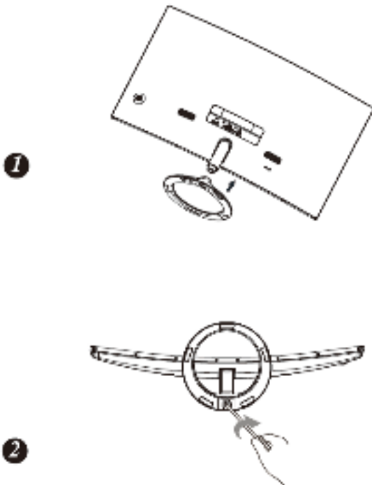
Figure.1. Installing and Removing the Base
