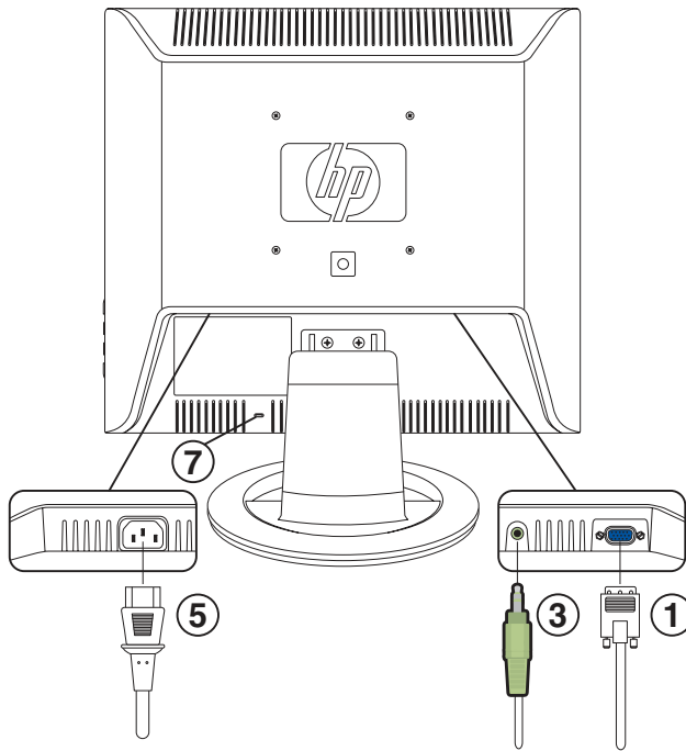
Connecting cables on the vs monitor
