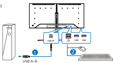
USB hub
