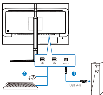
USB hub
