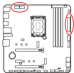
CPU_PWR1~2
