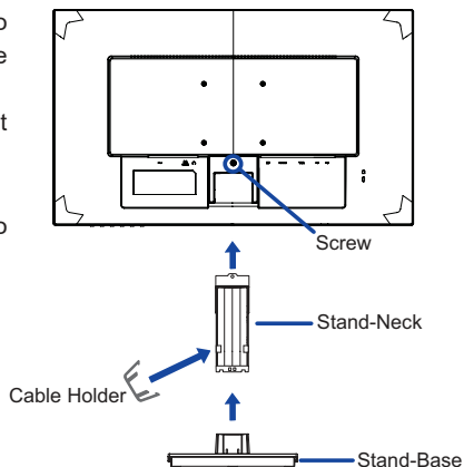
Thumb screw for Stand-Base fixing
