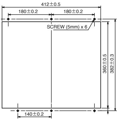
Panel aperture dimensions
