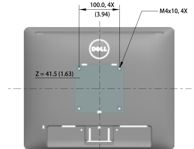
Back view of Monitor without stand
