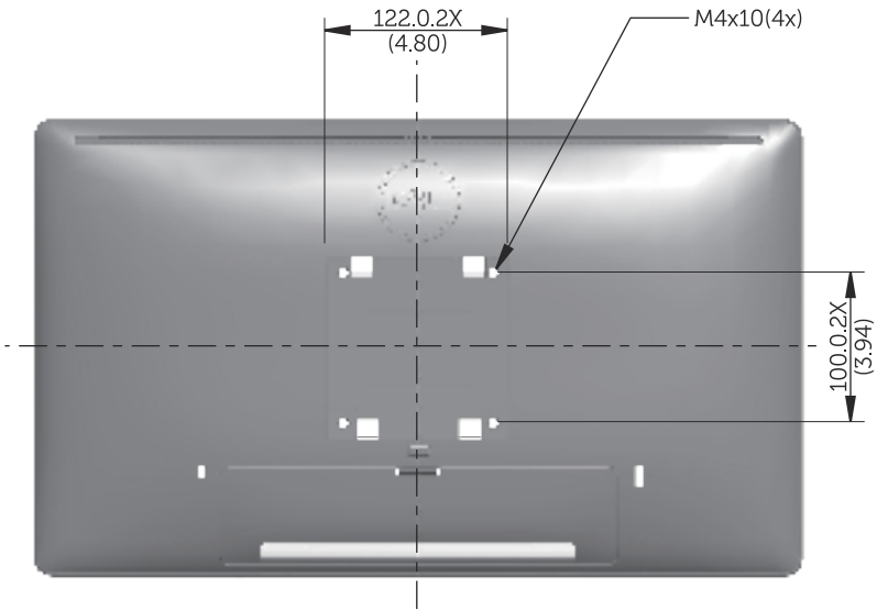
Back View of Monitor without stand
