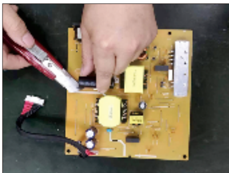
S18-3 Cut into the bottom of bulk cap. and pullit up carefully.
