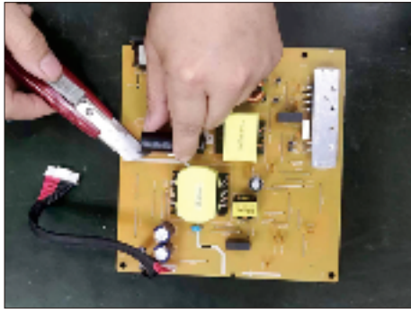
S18-2 Ensure cutting path within the glue, don't touch bulk cap. or PCB.
