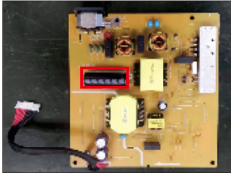
S18-1 Cut the glue between bulk cap. and PCB with a knife.
