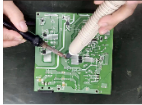
S18-5 Lift the bulk cap. up and away from the PCB.
