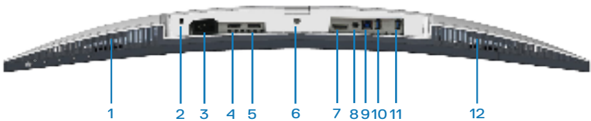
Bottom view without monitor stand
