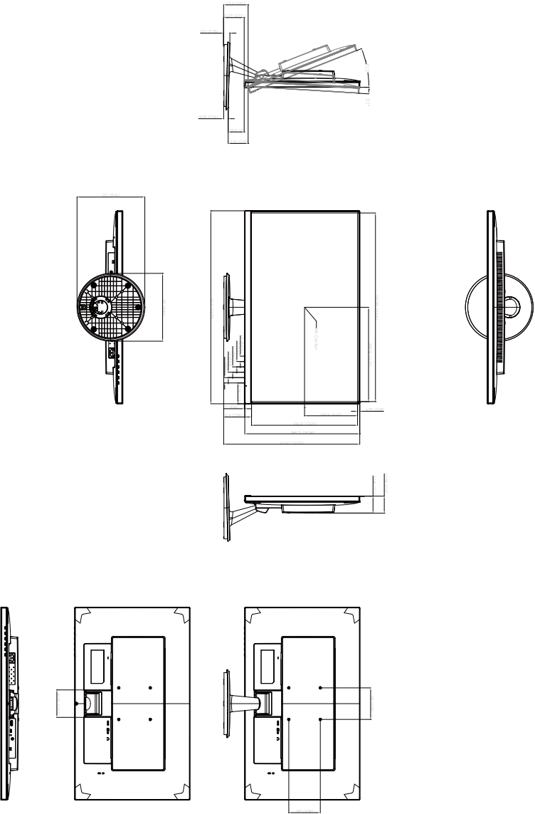
ASUS VA27DCP Outline Dimension Unit: mm (inch)
