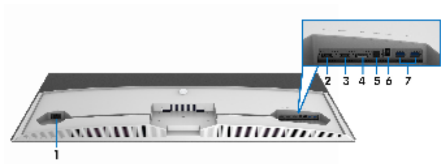
Bottom view without monitor stand
