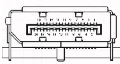
20-pin color display signal cable
